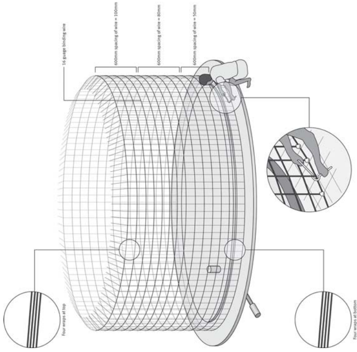
Fig 3: Wrapping the reinforcing wire
