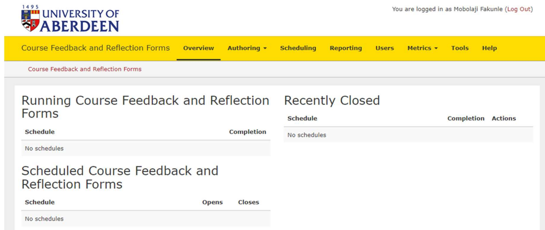
Figure 2: Dashboard Page
