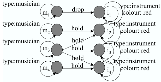
Figure 1: A scene graph involving eight objects
