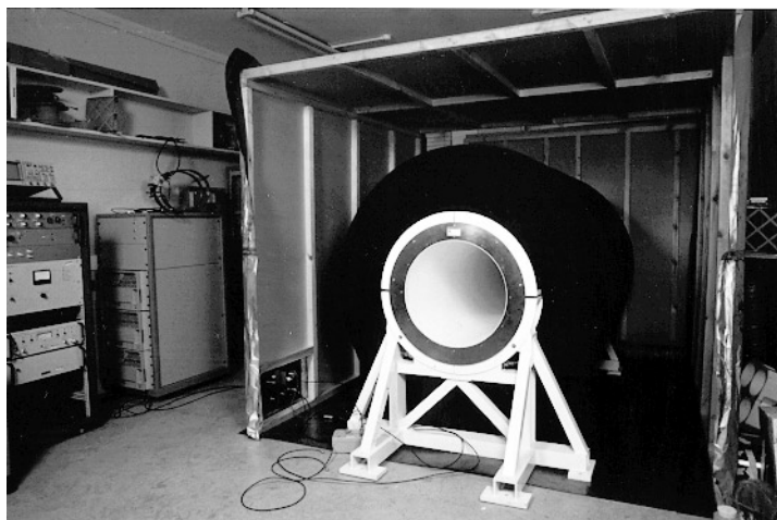
Figure 2. Photograph showing the whole-body FC-PEDRI imager, before the Faraday screen was completed. Not seen in the photograph are the RF coil assembly, the secondary magnet power supply and the NMR console.
