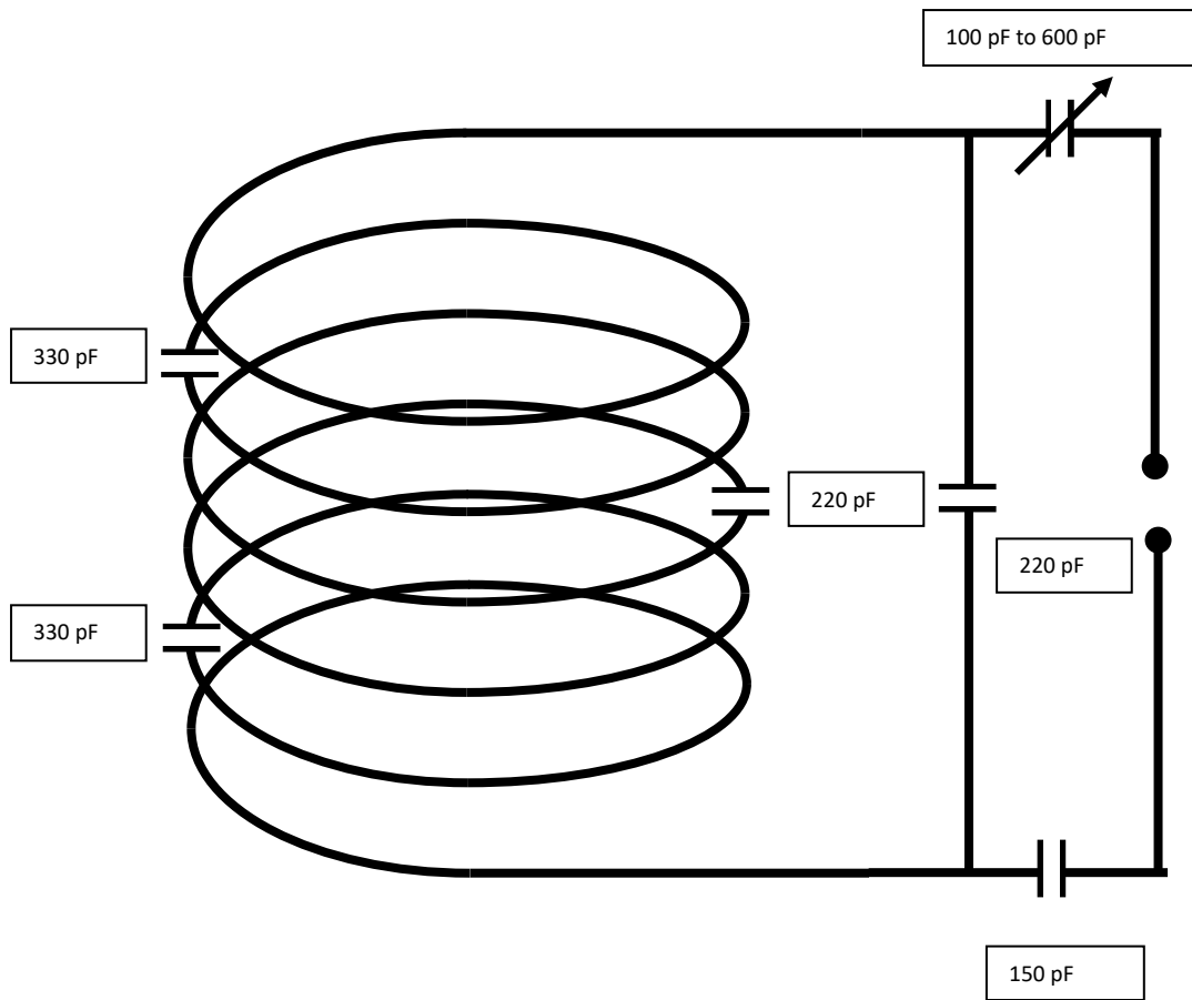
Figure 1. A schematic layout of the unilateral breast coil circuit.
