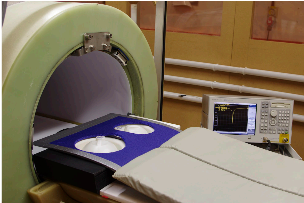
Figure 4. Tuning and matching of the bilateral RF coil before an imaging test, with \text{MnCl}_2 phantoms, in the 0.2 T FFC-MRI scanner. The coil box is mounted on the dedicated couch that would increase the space in the bore available to a subject.
