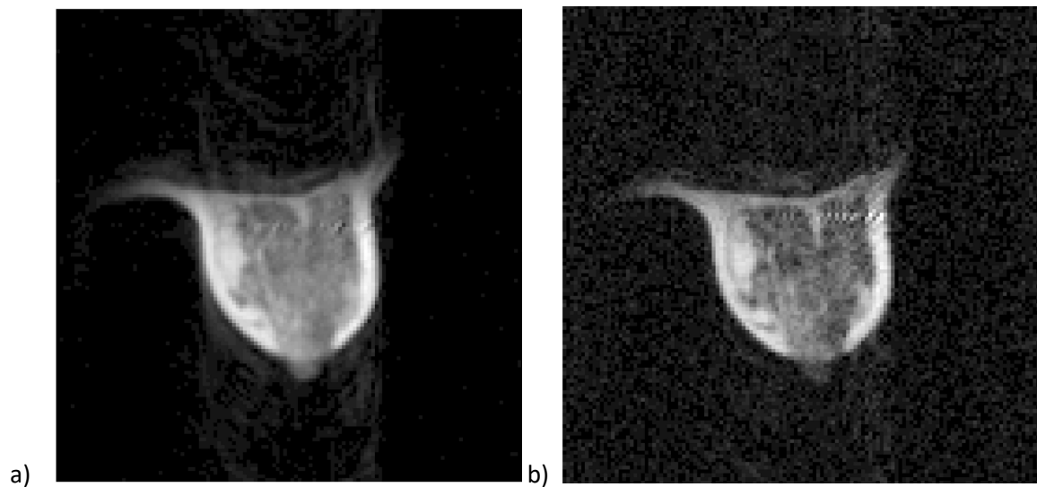
Figure 5. FFC-MRI sagittal images, from the unilateral coil, of the left breast of a healthy volunteer with evolution fields of a) 200mT, b) 1 mT
