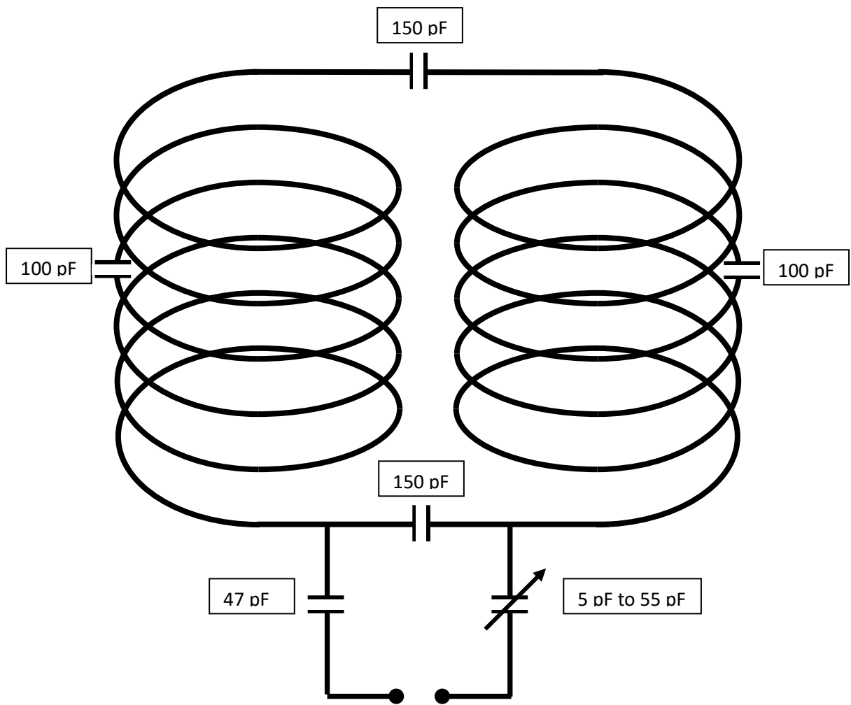
Figure 2 A schematic layout of the bilateral breast coil circuit.
